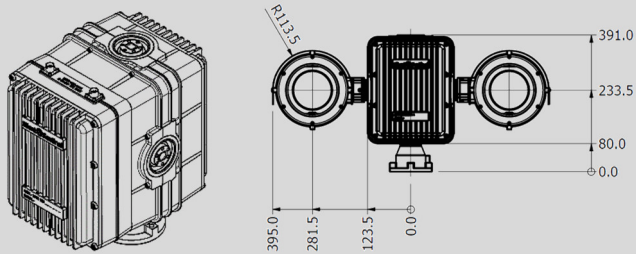
HT07 Camera Housing
